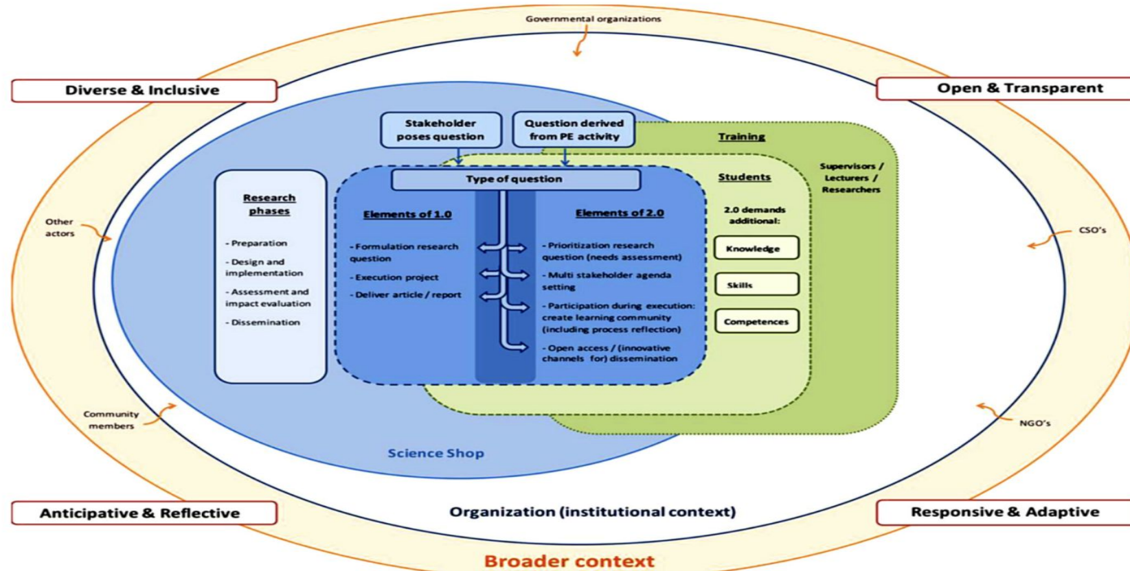
Fig. 3. Framework.
